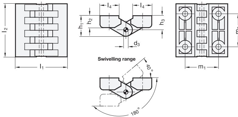
ELESA original design CFA.
