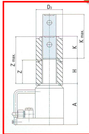
B Lifting cylinder with extension kit
