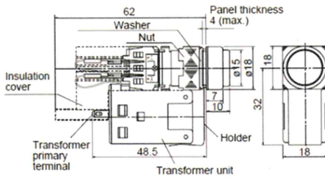
Pilot light/with transformer AH164-Z□, AH165-Z□
