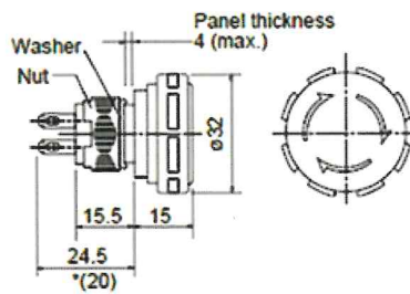
Pushbutton switch/ Push-lock, turn-reset AH164-VR□, AH165-VR□
