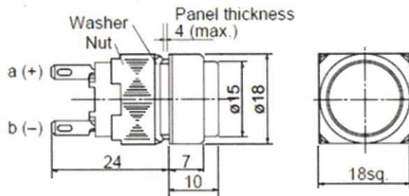
Pilot light/with transformer AH164-Z□, AH165-Z□
