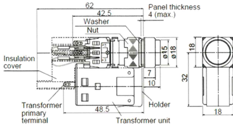
Pushbutton switch AH164-TF□, AH165-TF□
