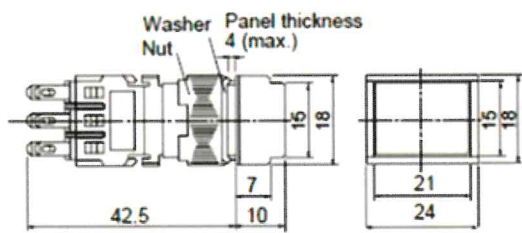
Pushbutton switch AH164-TF□, AH165-TF□
